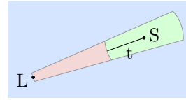
Figure 3. Sketch of the accuracy evaluation given a single scan point, S , measured from the laser scanner position L , with evaluation threshold t . Reconstruction points within the green region are accurate, points in the red region are inaccurate, and points in the blue region are unobserved.
